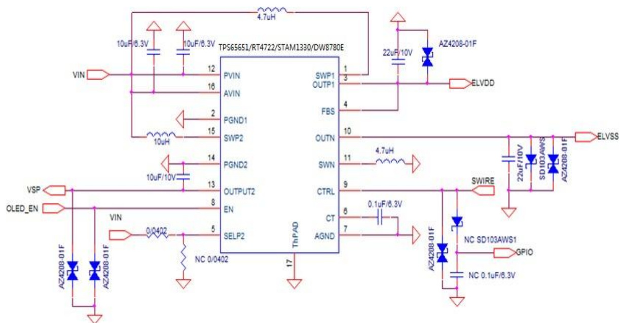
5.1.2 Application circuit:
